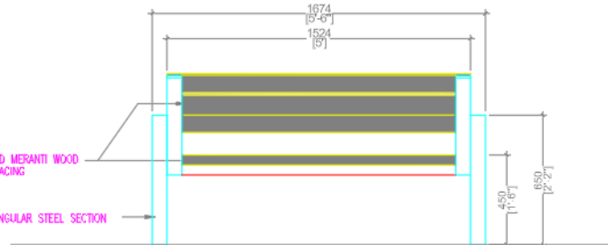
REAR ELEVATION
